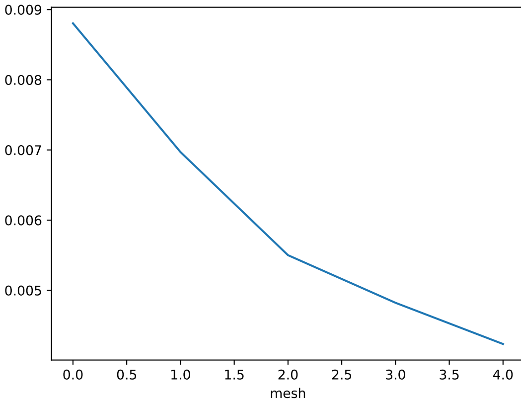
Error estimate over each mesh for z = 2.05
