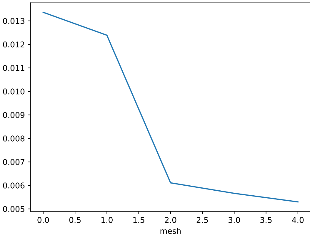
Error estimate over each mesh for z = 2.1499999999999995
