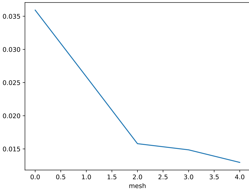
Error estimate over each mesh for z = 2.5999999999999998
