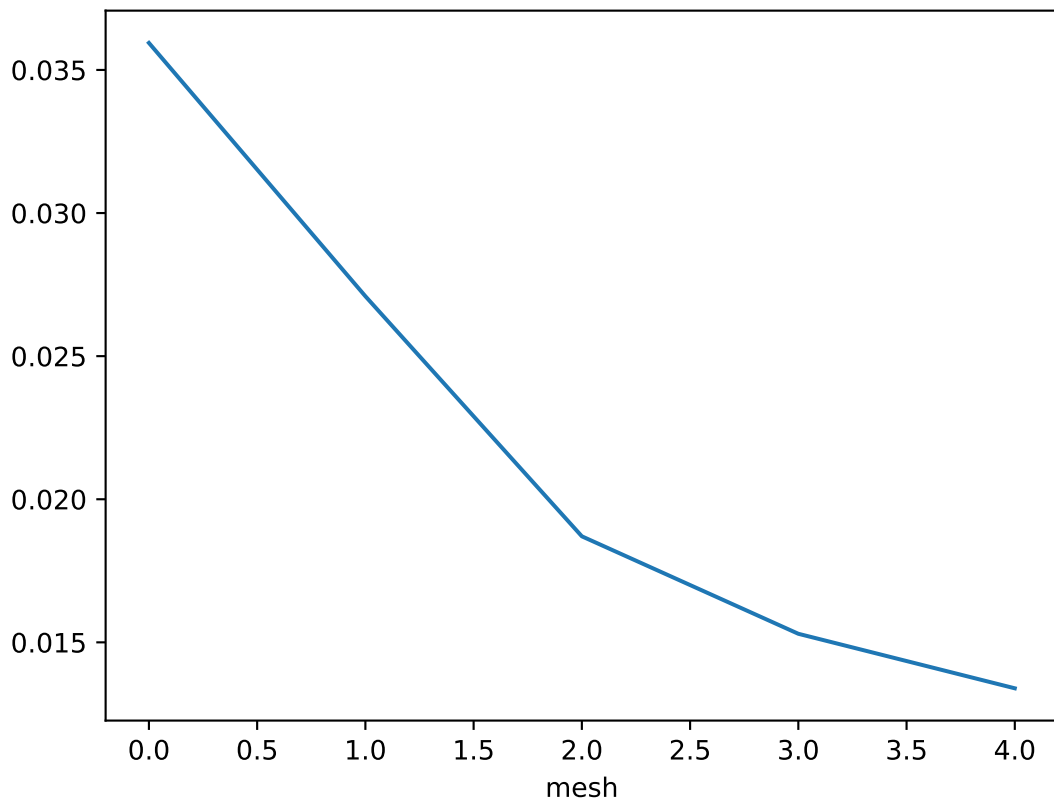
Error estimate over each mesh for z = 2.7999999999999997
