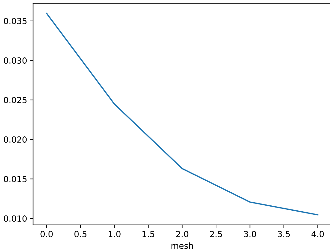
Error estimate over each mesh for z = 2.8999999999999997
