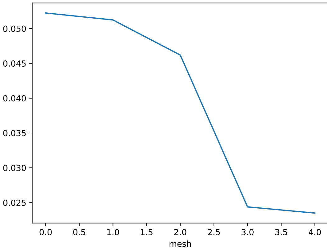
Error estimate over each mesh for z = 3.24999999999999956
