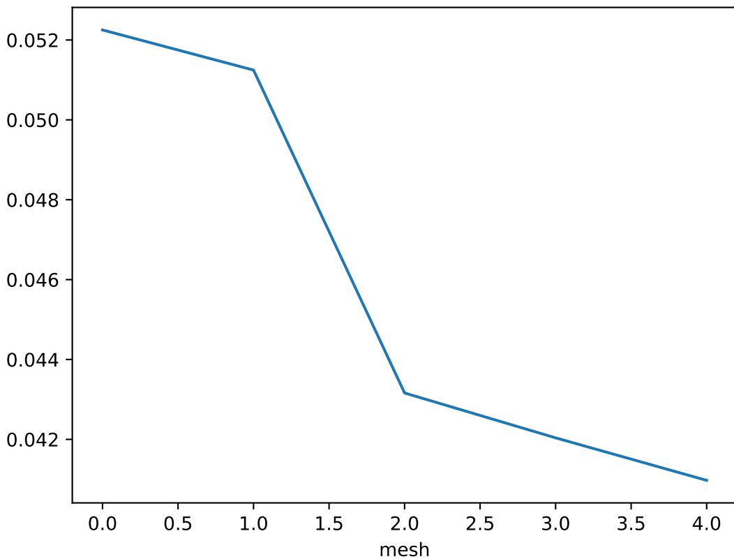
Error estimate over each mesh for z = 3.29999999999999954
