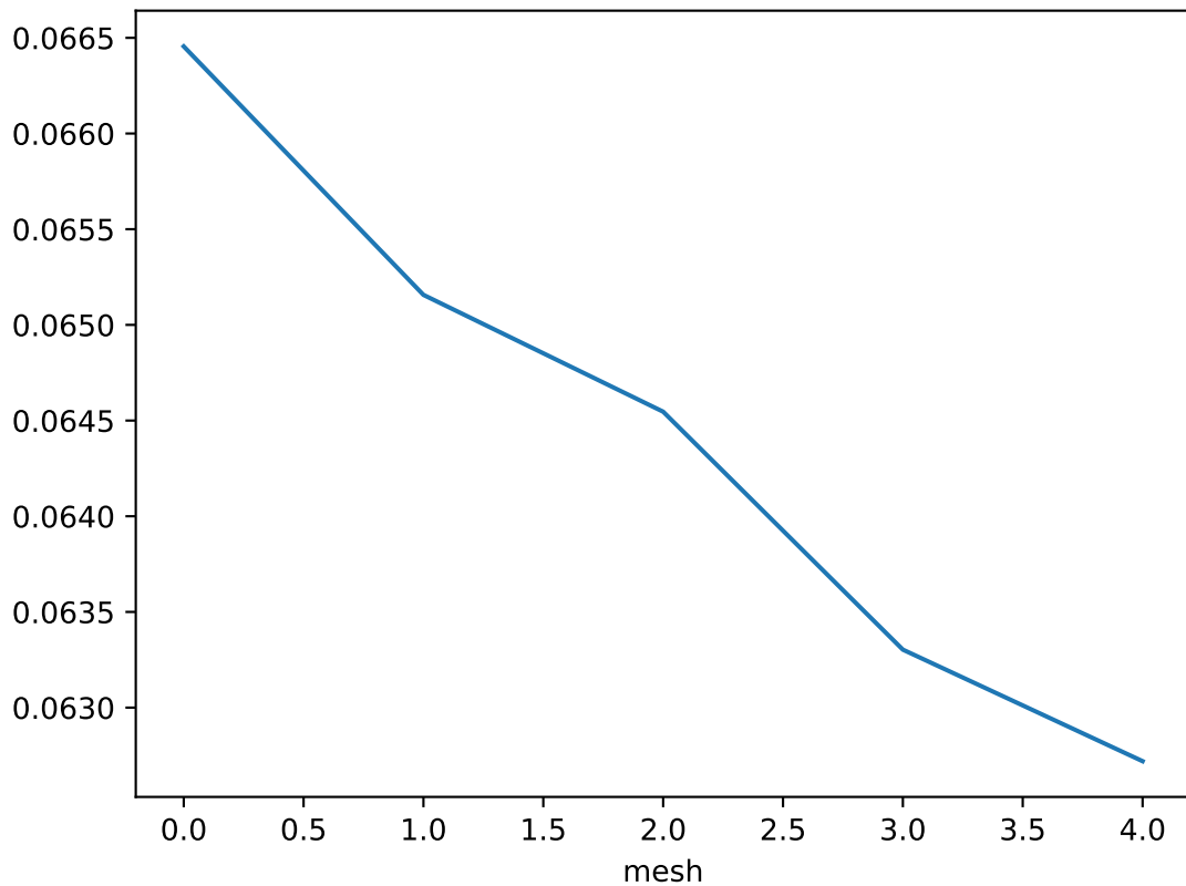
Error estimate over each mesh for z = 3.3999999999999995
