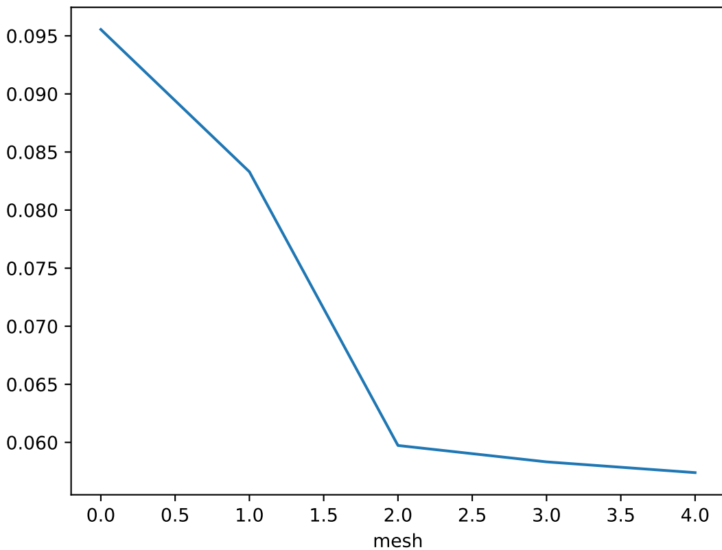
Error estimate over each mesh for z = 3.59999999999999943
