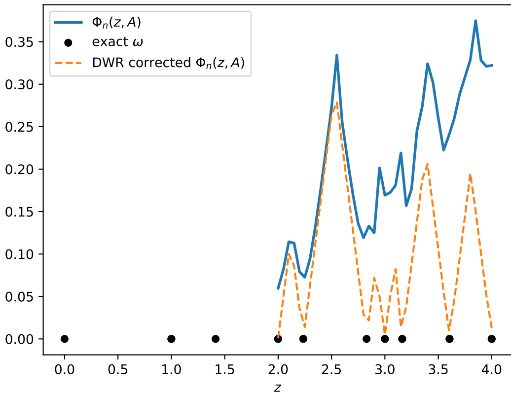
Approximations of \Phi_n(z, A) and \omega ( N = 32 )
