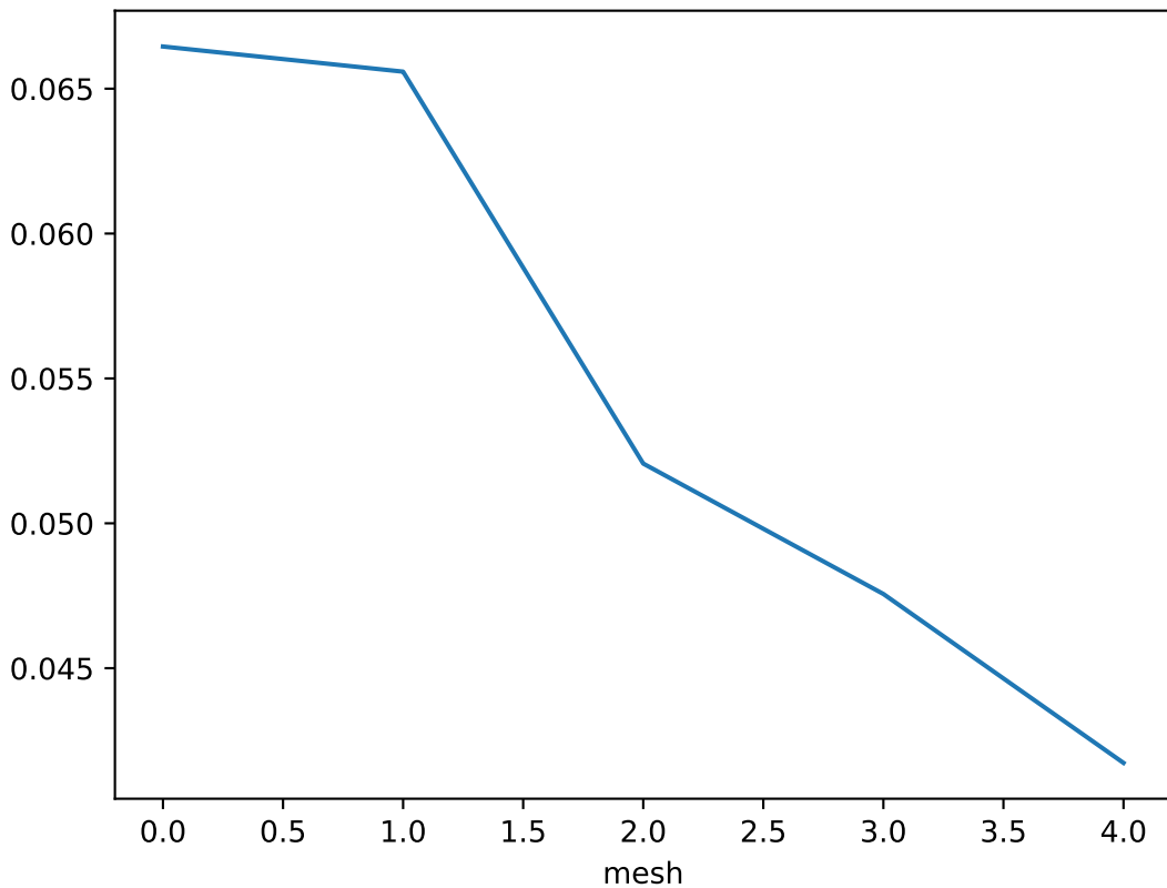
Error estimate over each mesh for z = 3.40000000000000012
