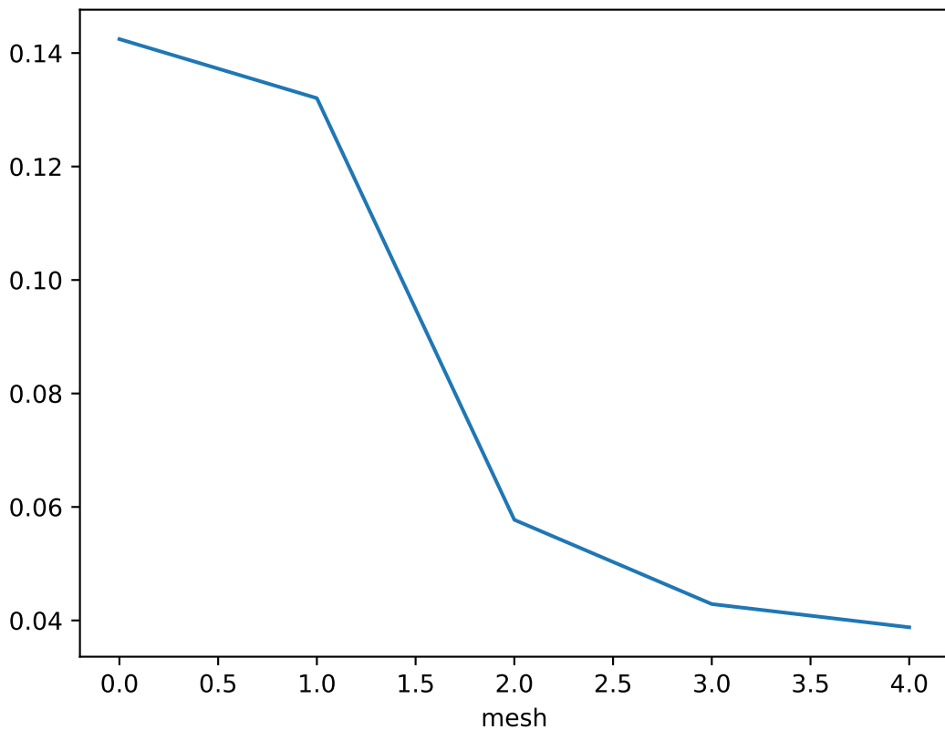
Error estimate over each mesh for z = 4.0
