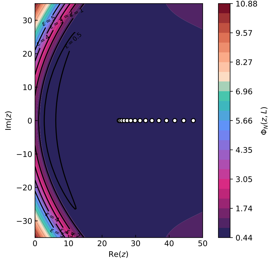
1D advection--diffusion, Hermite 3 , N = 128
