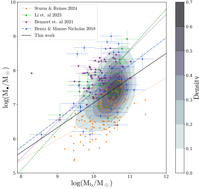
Figure 3. Comparison between our best-fit power law scaling relation between M_{SE} and M_b (mergers+non-mergers, first row of Table 1) and previously published M_\bullet – M_b scaling relations from AGN broad lines and photometric bulge mass. Our sample of 2,219 Type 1 AGN are plotted as 2D contours corresponding to the Gaussian kernel density of points and our scaling relation is the black line. The data points and scaling relations of Bentz & Manne-Nicholas (2018) (blue triangles), Bennert et al. (2021) (purple diamonds), Li et al. (2023) (green squares), and Sturm & Reines (2024) (orange circles) are shown for comparison. Descriptions of each sample and scaling relation parameters are in Table 1. The SMBH masses from this are under-massive relative to all published scaling relations aside from Sturm & Reines (2024).
