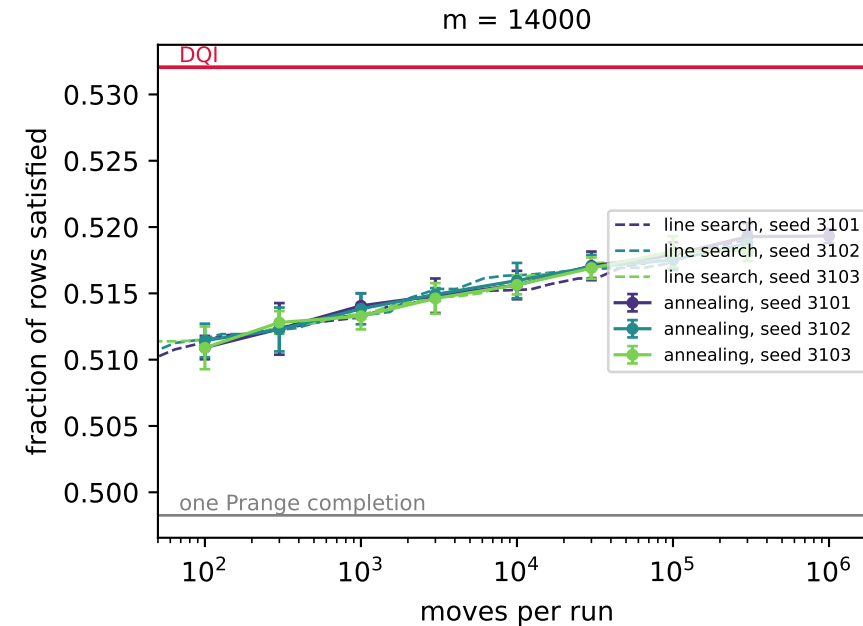
alternant max-agreement (AMA), s = 6 : annealing (mean and spread over chains) and line search (mean over chains)
