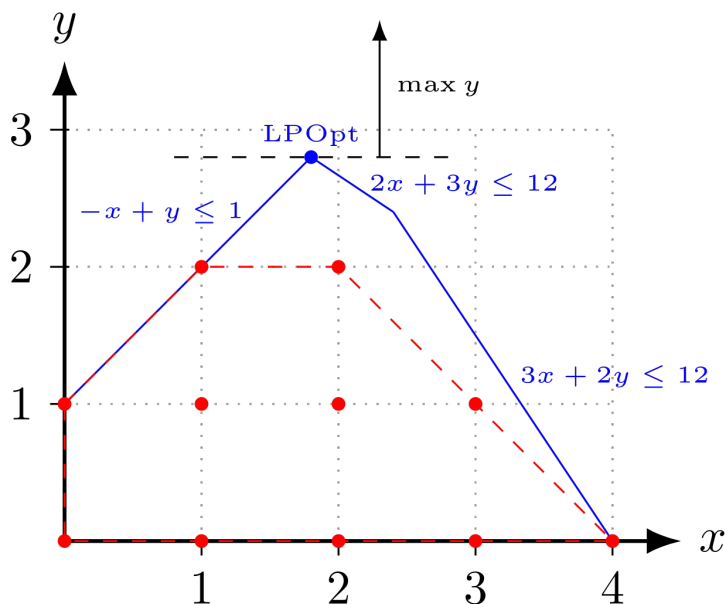
Figure 2: Polytopes of all feasible integer points and of the LP relaxation to the integer linear program \max\{y \mid -x + y \leq 1; 3x + 2y \leq 12; 2x + 3y \leq 12; x, y \in \mathbb{Z}_+\} . (CC-BY; Fanosta – derivative work based on “IP polytope with LP relaxation.png” by Sdo.)
