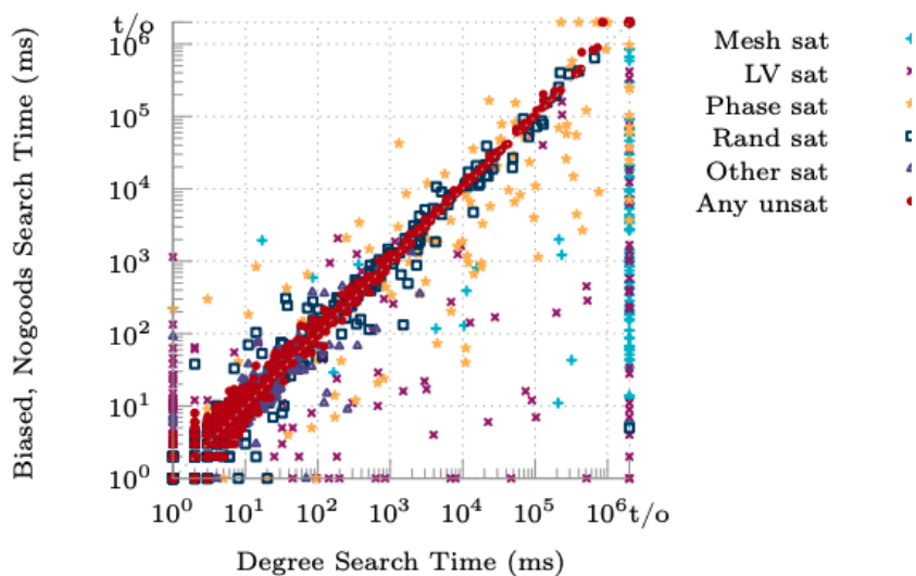
Figure 4: Degree search time versus biased, nogoods search time, across several instance families (log-log axes; t/o marks the timeout boundary).
