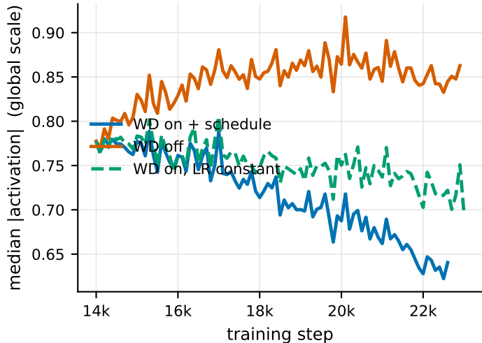
Weight decay drives the global decline
