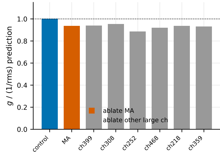
Gradient obeys g \propto 1/\text{rms} ; MA on the line
