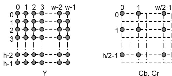
4) YCbCr 4:2:0 (co-sited)
