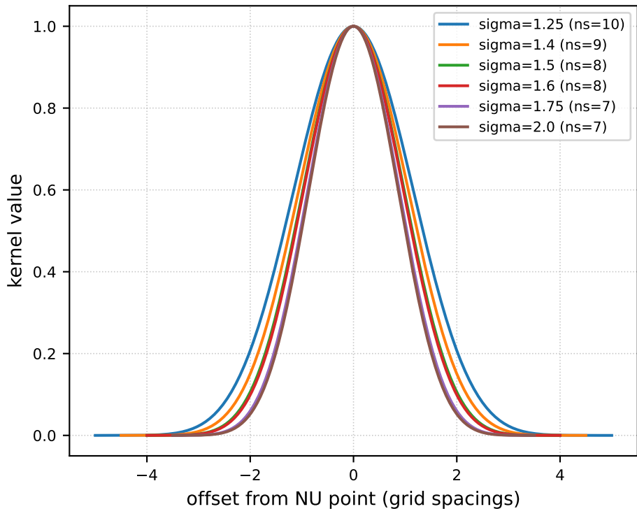
ES spreading kernel shrinks as sigma increases (tol=1e-06)
