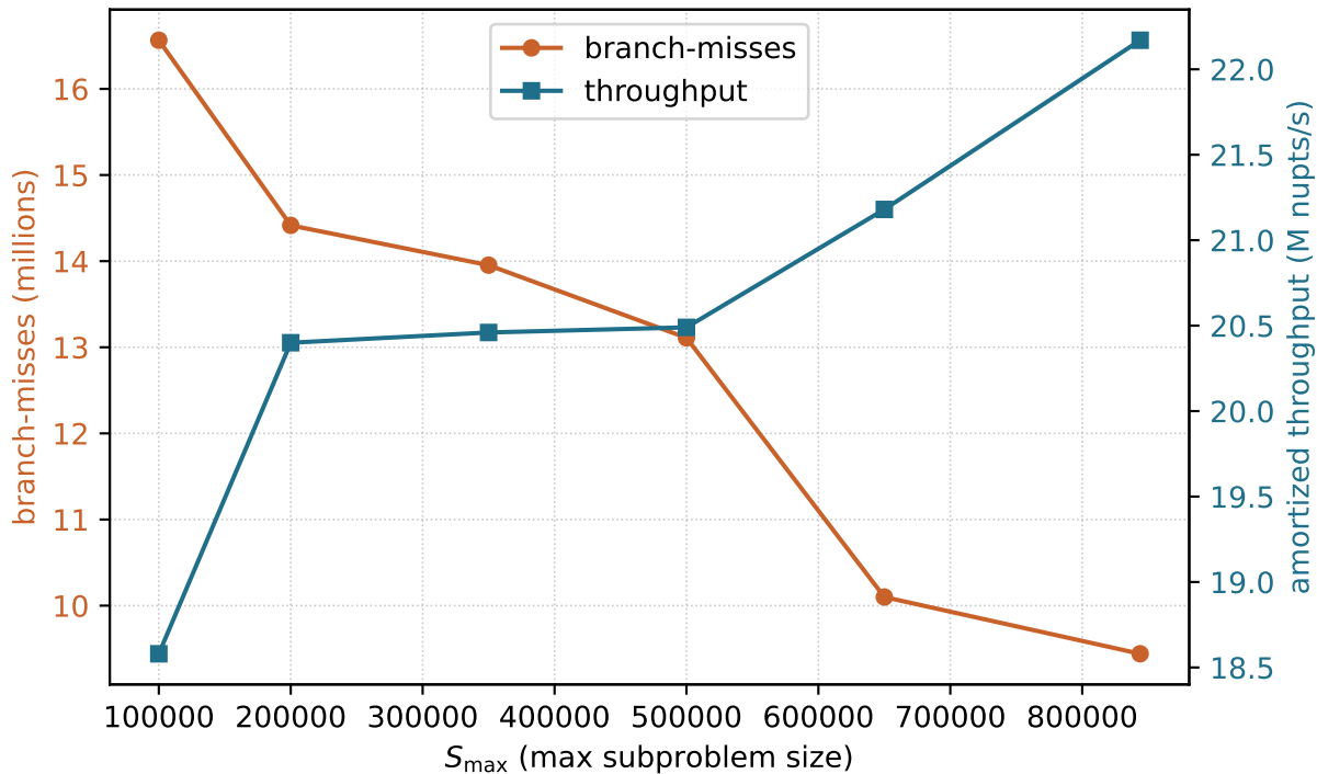
S_{\max} vs. branch-misses and throughput (illustrative trend)
