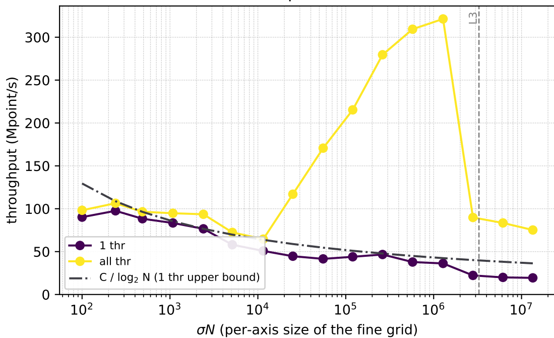
dim=2, prec=double
