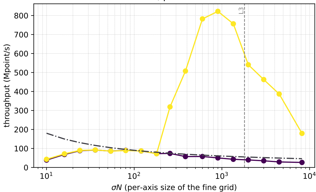
dim=3, prec=double
