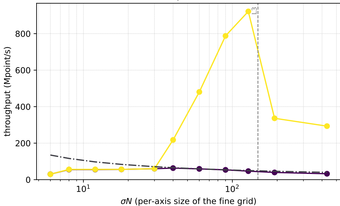
dim=3, prec=double
