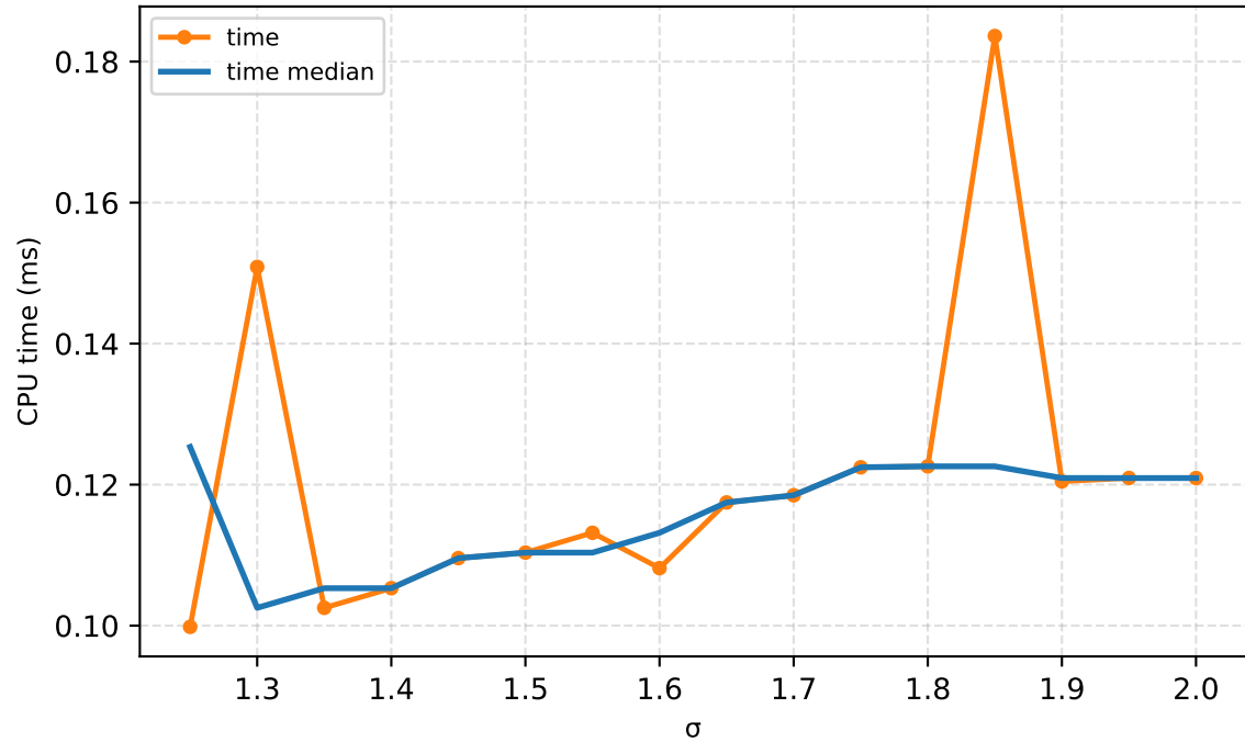
1D tol=1e-08 double \rho=0.5
