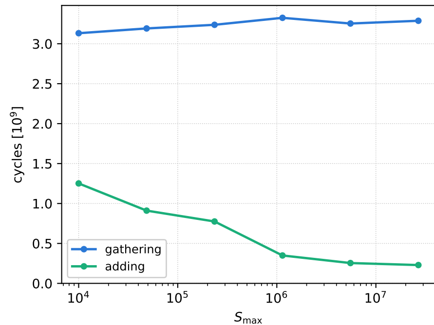
\rho = 1 , 1 thread
