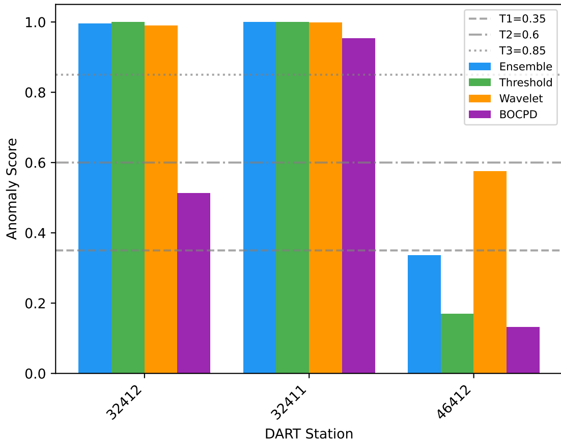
Chile 2010 (Mw 8.8): Per-Station Anomaly Detection Scores
