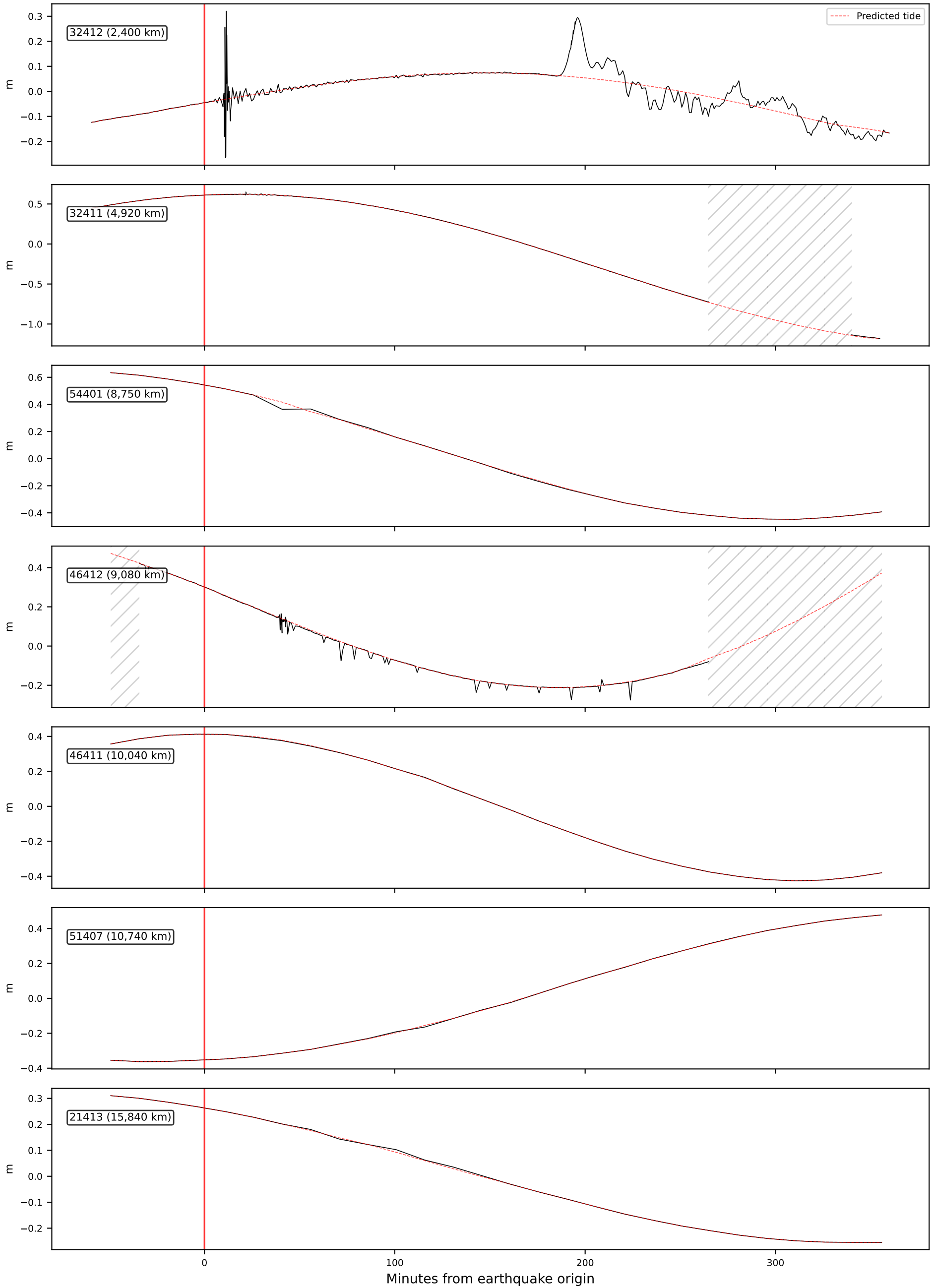
Chile 2010 (Mw 8.8): Raw Bottom Pressure Records (De-meaned)
