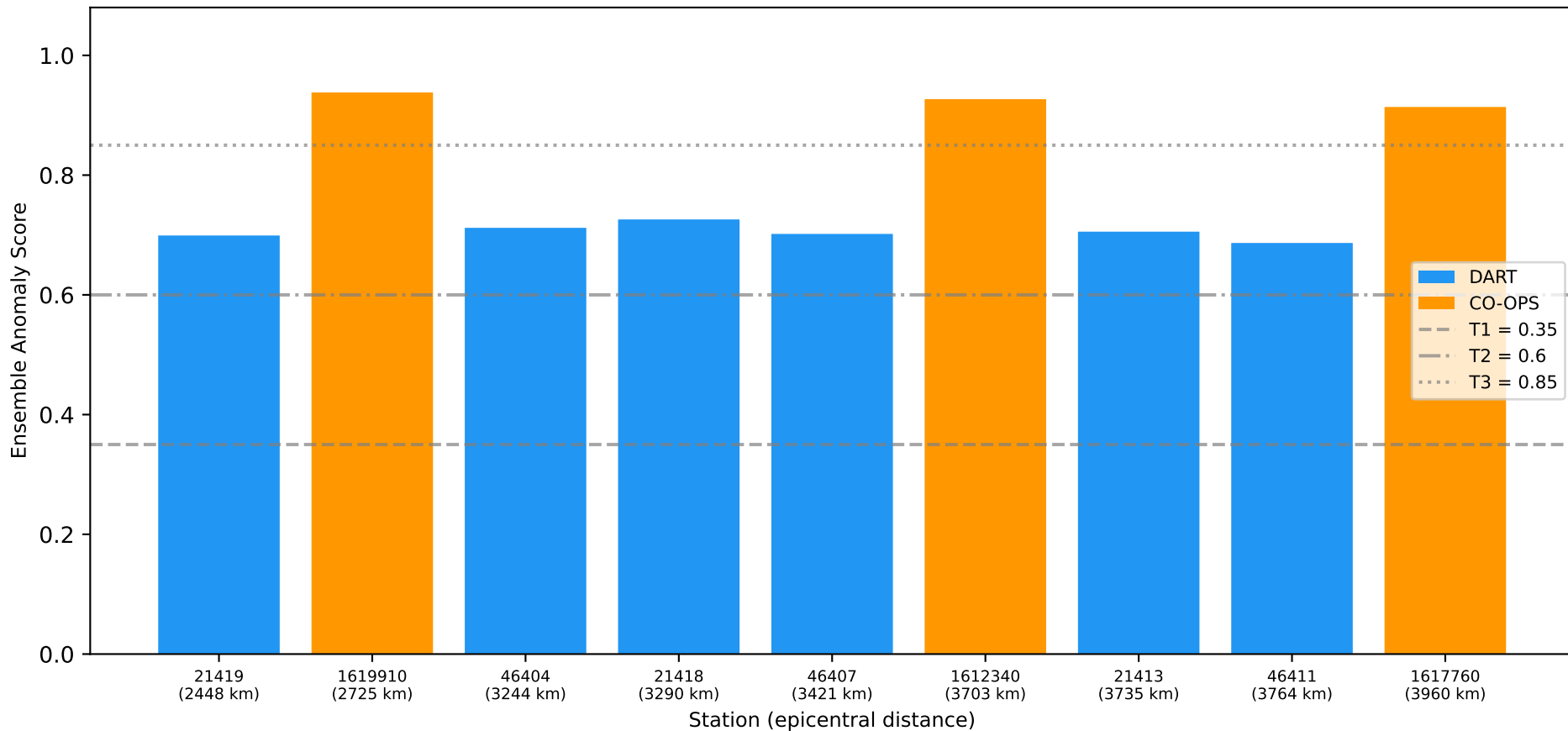
Physics Simulation: Large Tsunami (M8.5 Aleutian) (6 DART and 3 CO-OPS Stations)
