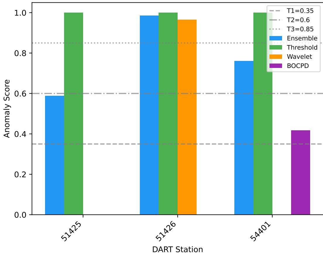
Samoa 2009 (Mw 8.1): Per-Station Anomaly Detection Scores
