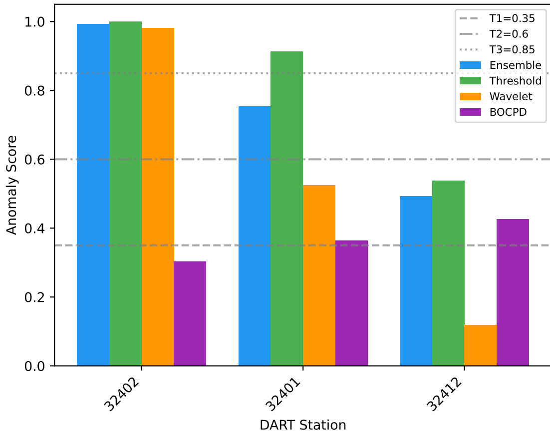
Illapel 2015 (Mw 8.3): Per-Station Anomaly Detection Scores
