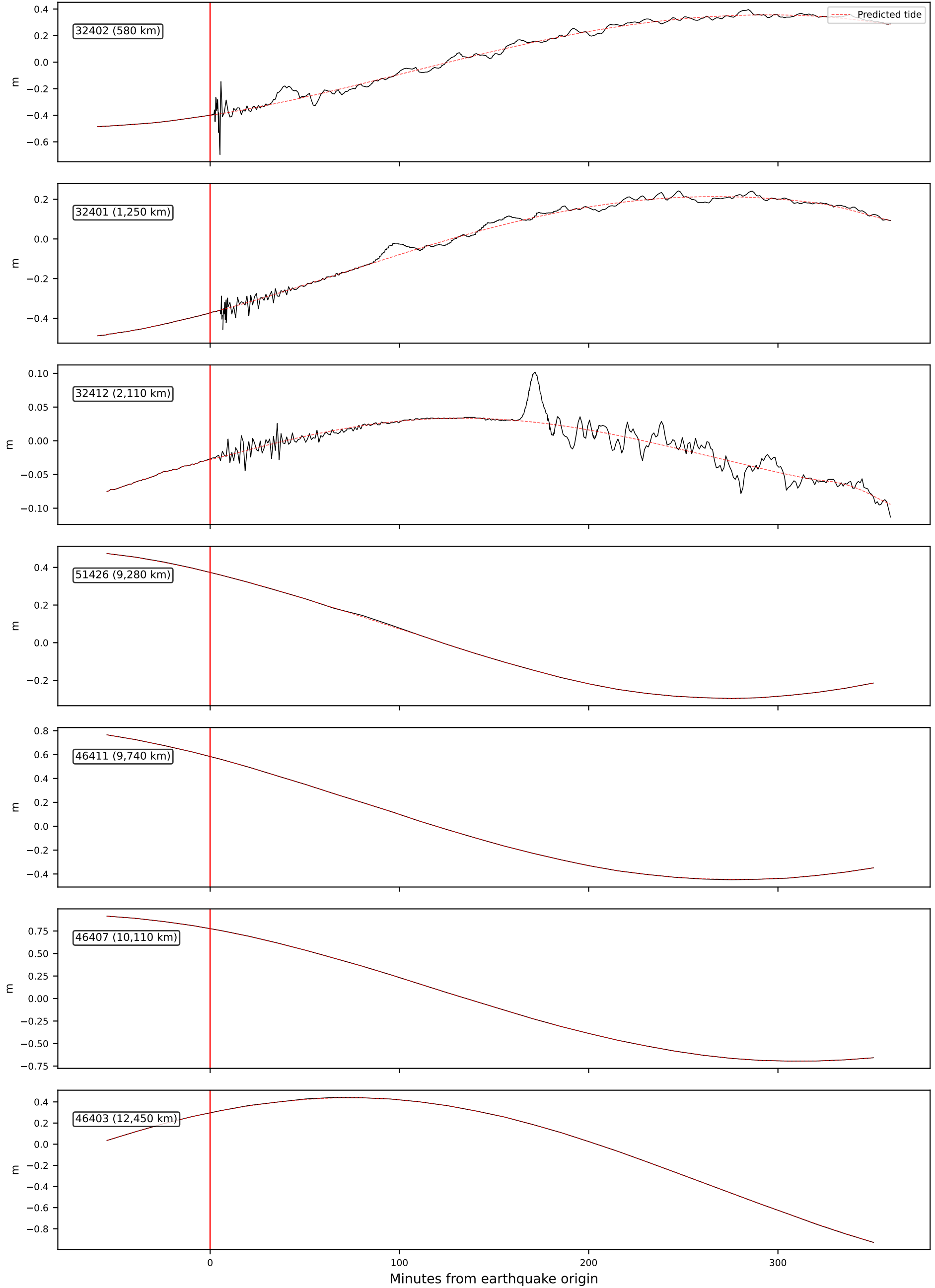
Illapel 2015 (Mw 8.3): Raw Bottom Pressure Records (De-meaned)
