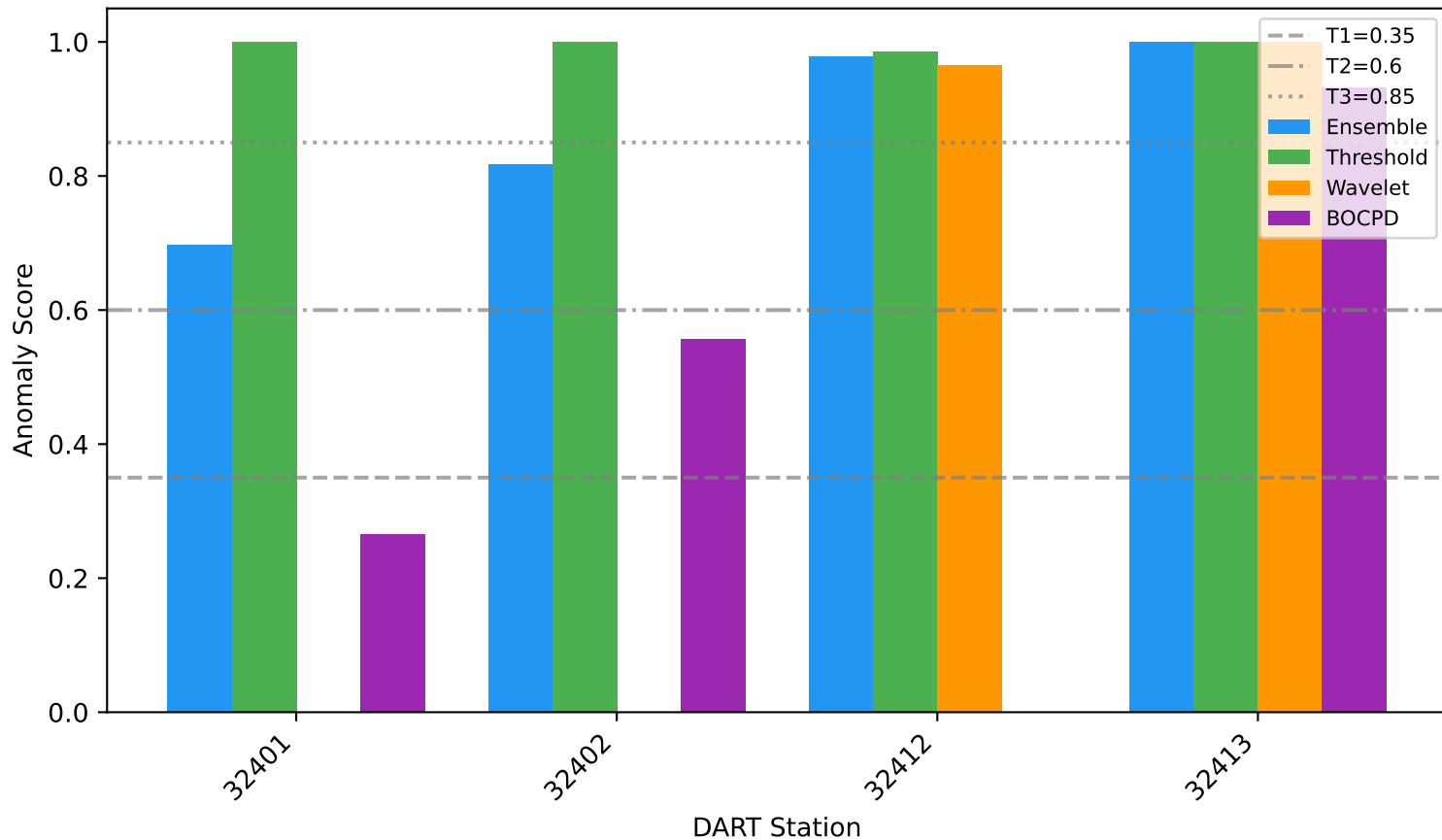
Iquique 2014 (Mw 8.2): Per-Station Anomaly Detection Scores
