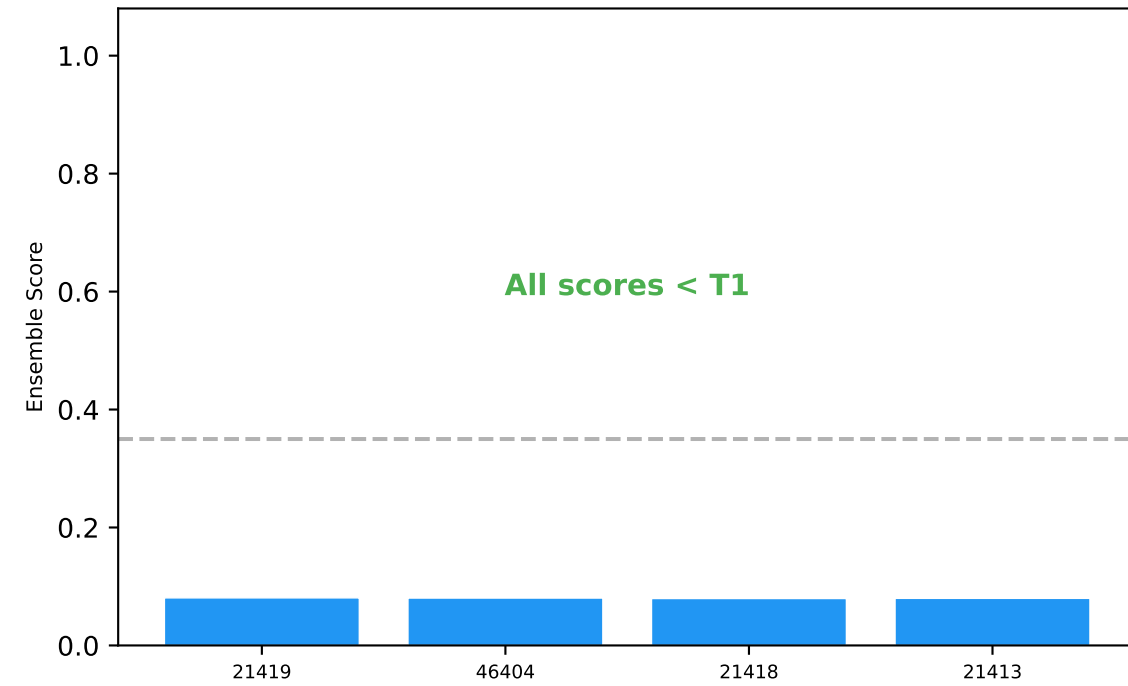
(b) Moderate Earthquake (M7.0 Aleutian): No False Escalation
