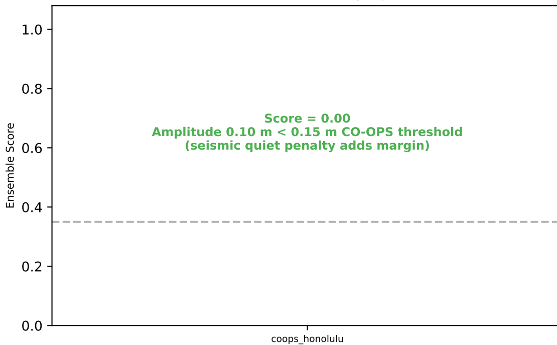
(c) Meteotsunami: Correctly Rejected
