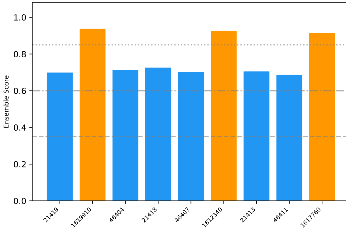
(c) Meteotsunami: Correctly Rejected
