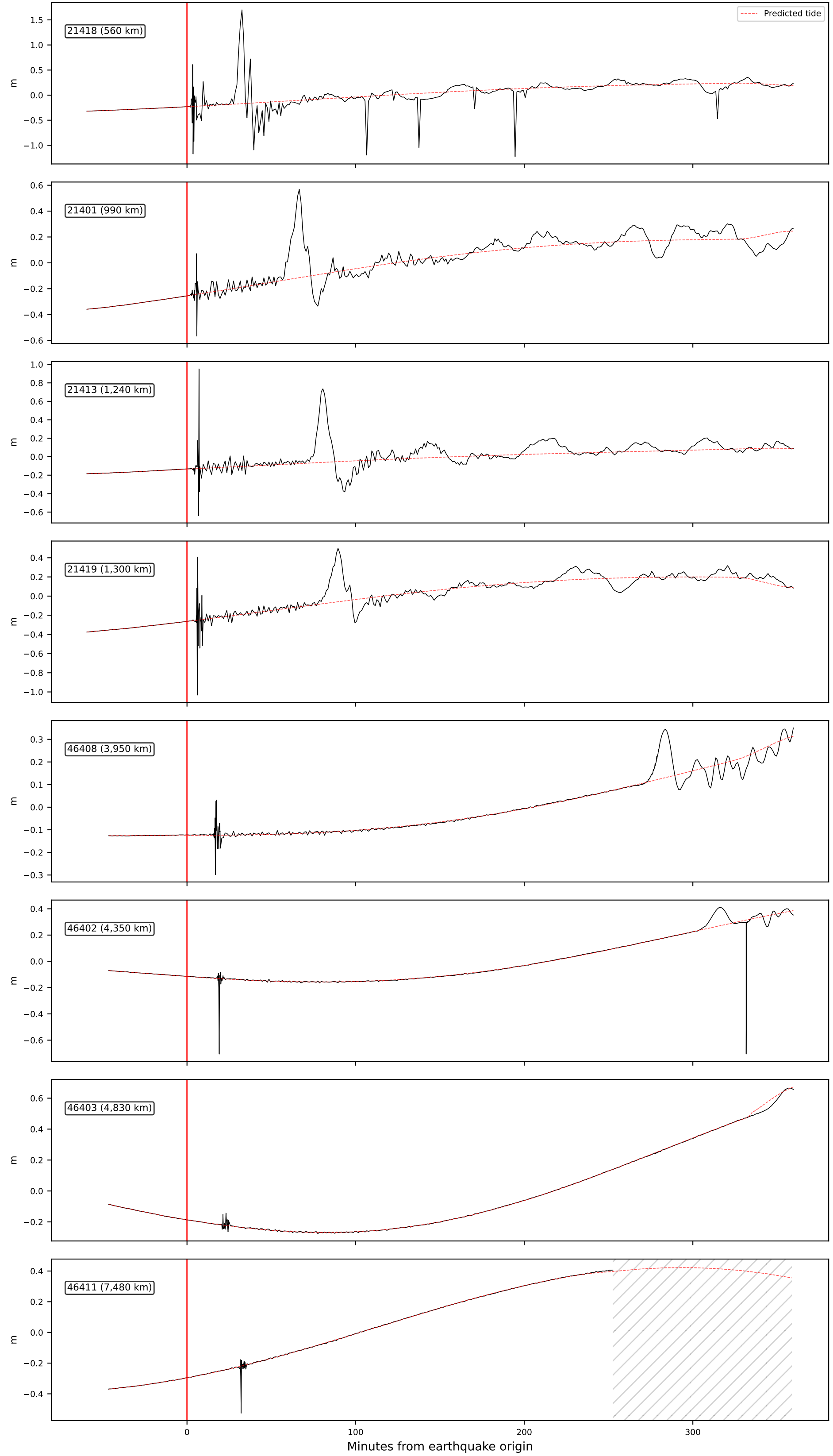
Tohoku 2011 (Mw 9.1): Raw Bottom Pressure Records (De-meaned)
