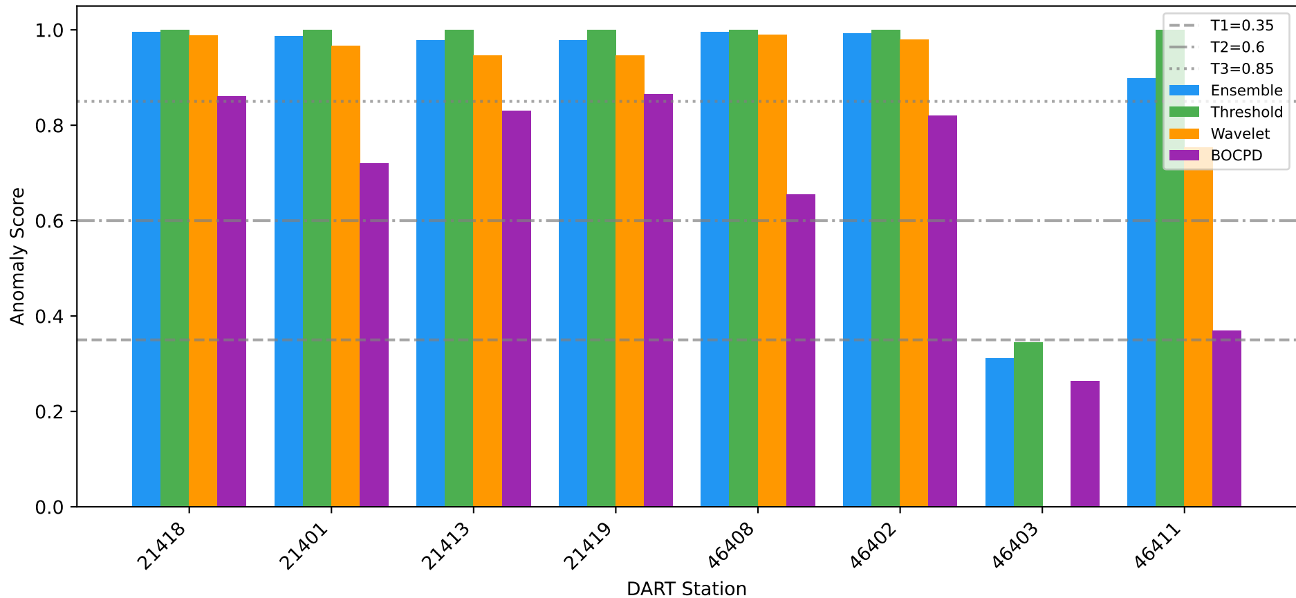
Tohoku 2011 (Mw 9.1): Per-Station Anomaly Detection Scores
