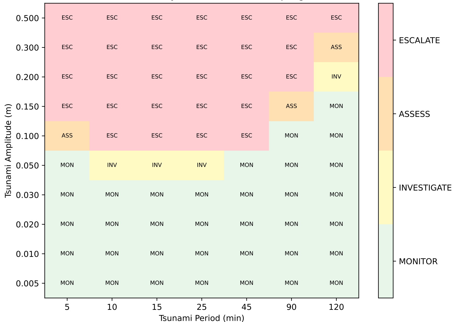
Detection Sensitivity: Noise 0.001 m, Sampling 60 s
