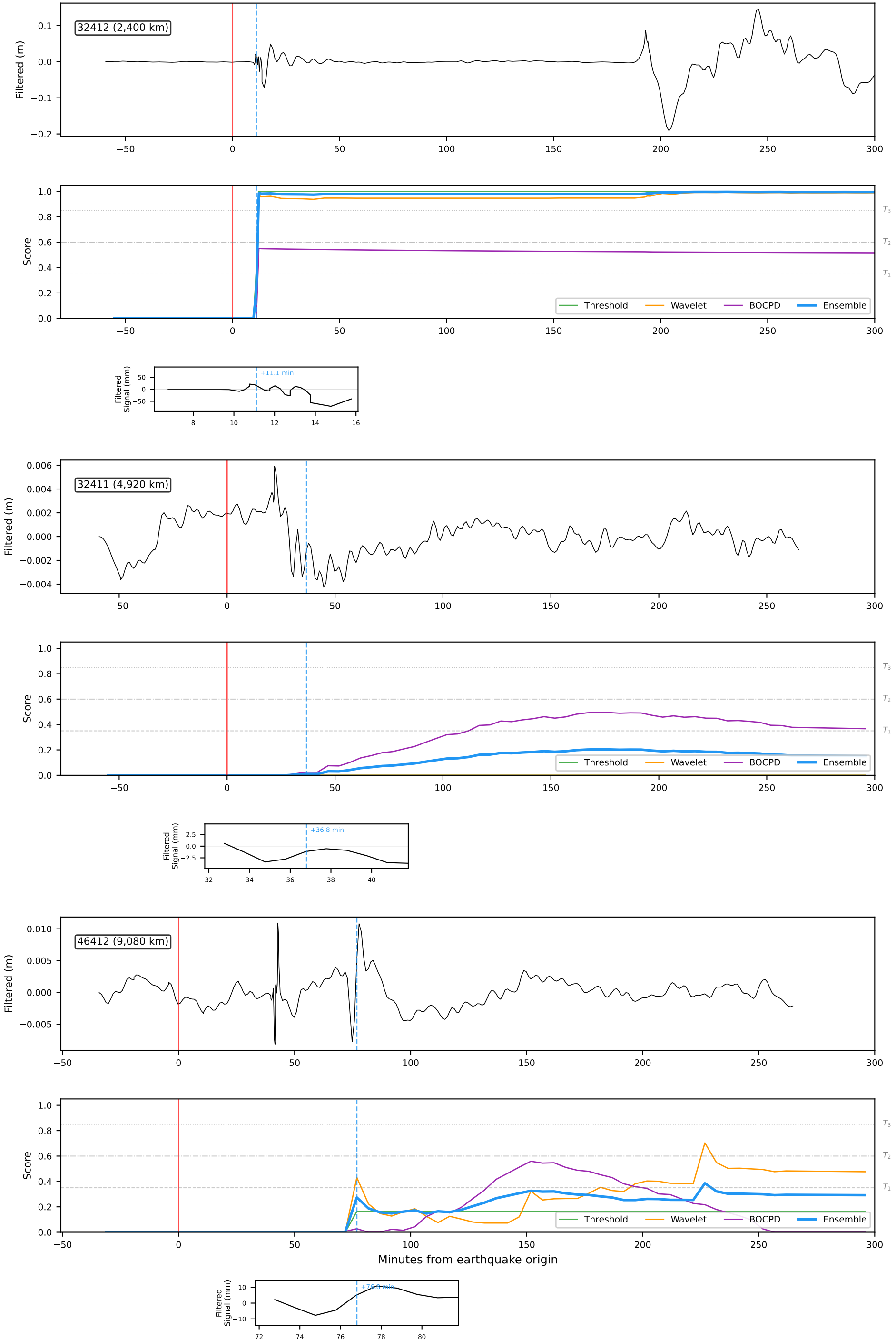
Chile 2010 (Mw 8.8): Bandpass-Filtered Residual and Detection Scores
