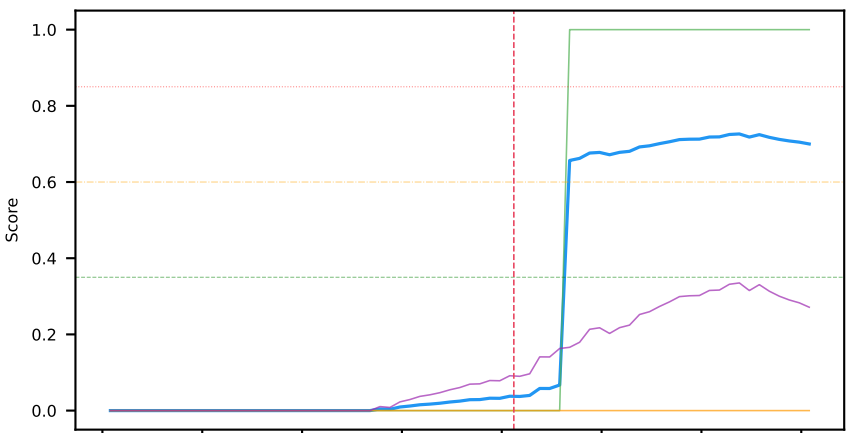
Score Evolution
