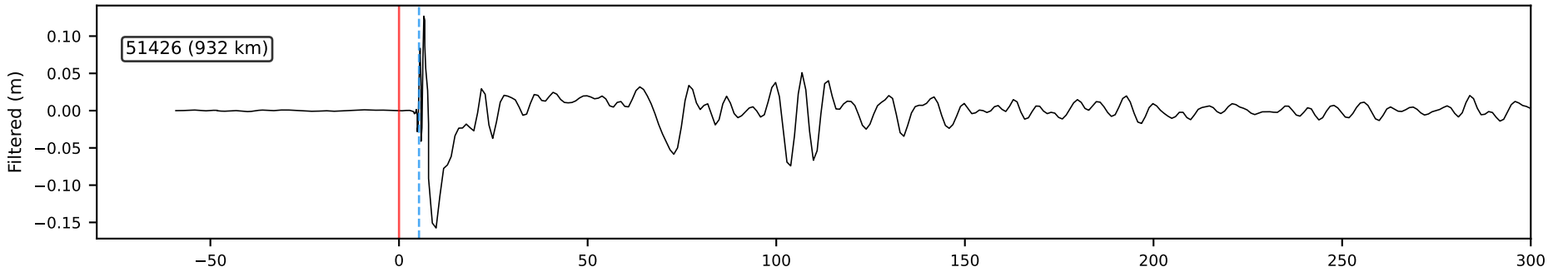
Samoa 2009 (Mw 8.1): Bandpass-Filtered Residual and Detection Scores
