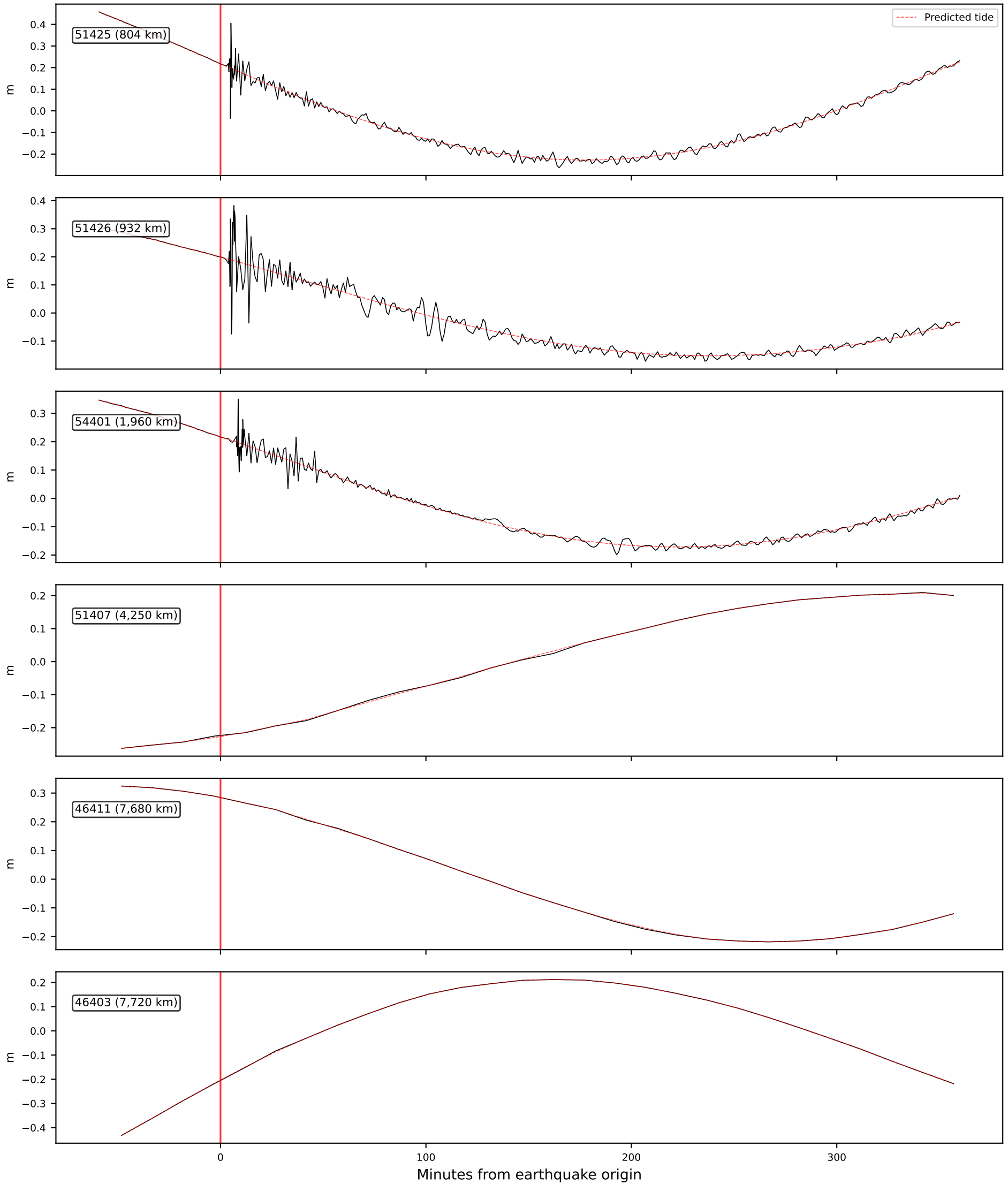
Samoa 2009 (Mw 8.1): Raw Bottom Pressure Records (De-meaned)
