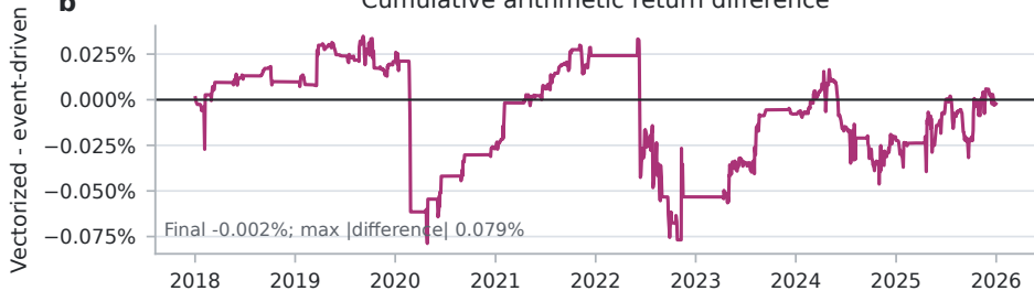
b Cumulative arithmetic return difference
