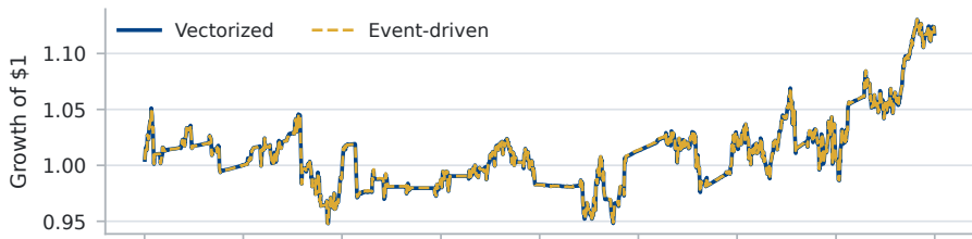
a Backtest-engine wealth at 13 bps
