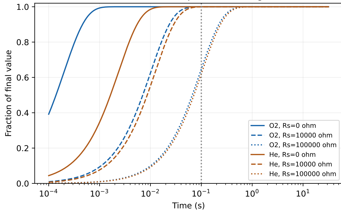
Nominal linear passive settling
