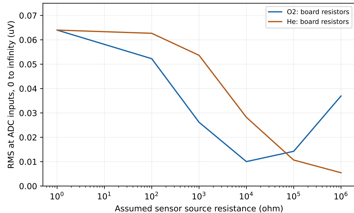
Board resistor thermal noise, 25 C
