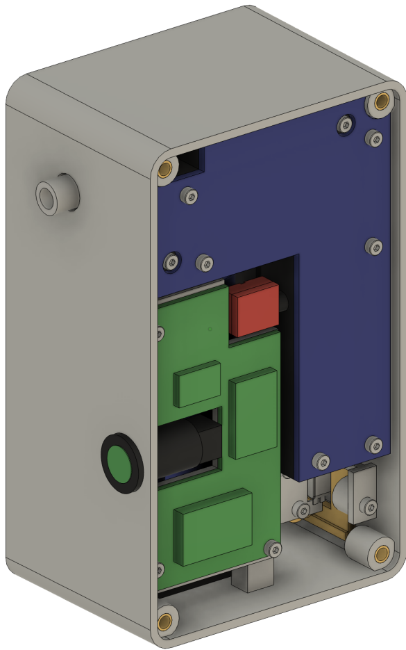
Rear cover hidden. Inspect the actual internal arrangement and rear-accessible retainers.
