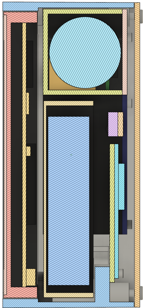
Screen left; rear cover right. Hatched cut shows display, pack and PCB depth clearances.
