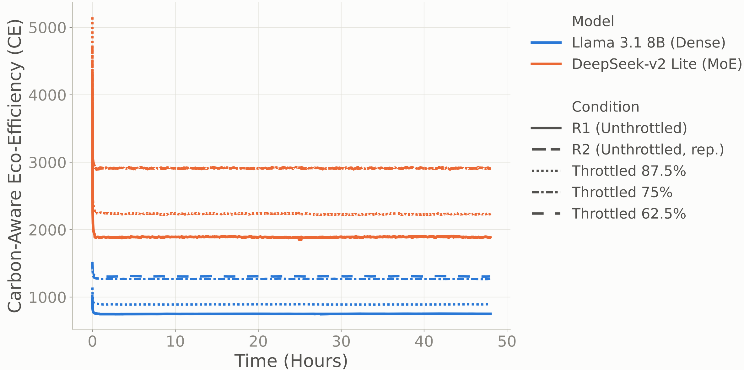
Llama 3.1 8B (Dense) vs DeepSeek-v2 Lite (MoE) — Carbon-Aware Eco-Efficiency (CE)
