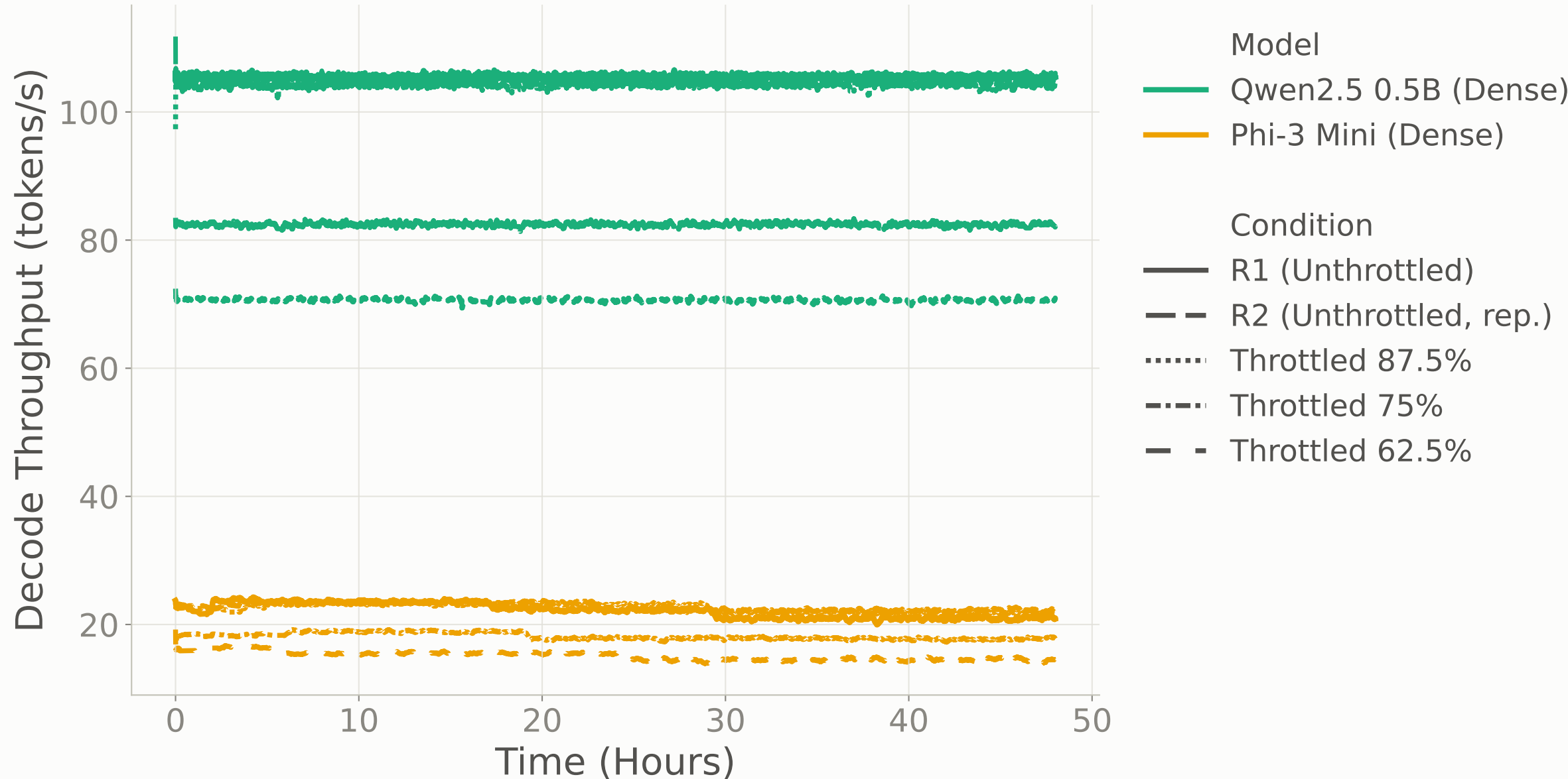
Qwen2.5 0.5B (Dense) vs Phi-3 Mini (Dense) — Decode Throughput (tokens/s)
