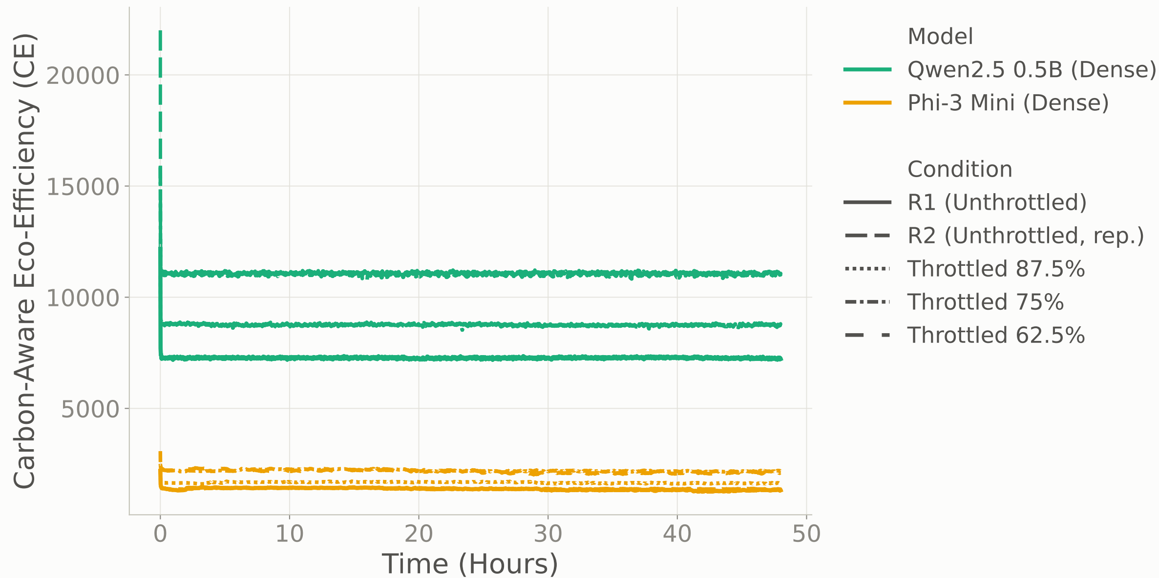
Qwen2.5 0.5B (Dense) vs Phi-3 Mini (Dense) — Carbon-Aware Eco-Efficiency (CE)
