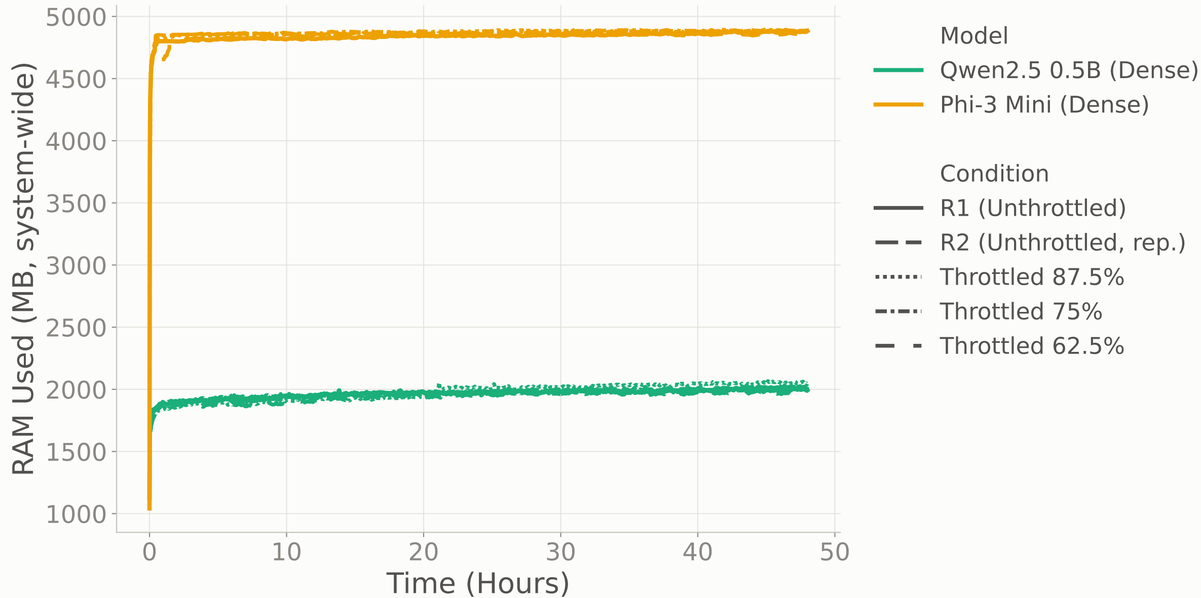
Qwen2.5 0.5B (Dense) vs Phi-3 Mini (Dense) — RAM Used (MB, system-wide)
