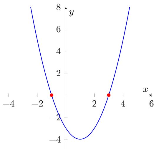
Figure 1: The graph of f(x) = x^2 - 2x - 3 crossing the x -axis at its two roots
