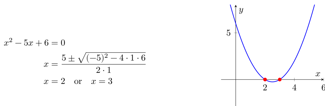
Figure 1: Solving x^2 - 5x + 6 = 0 and its graph, side by side
