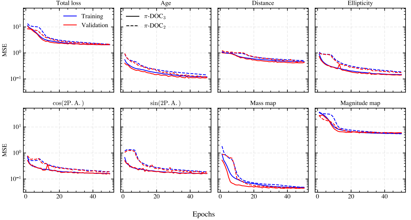
Fig. 3. Training curves for the two \pi -DOC variants considered in this study. Blue (red) lines correspond to the training (validation) MSE per output across epochs. The three-passband network converges faster and achieves lower overall MSE than its two-passband counterpart, although this difference is not substantial. We interpret this as a result of the larger (but not deeper) network capacity.
