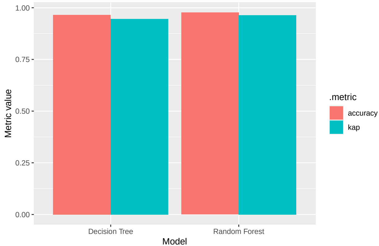
Model comparison
